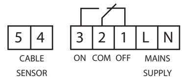
INTERNAL WIRING DIAGRAM CDC
